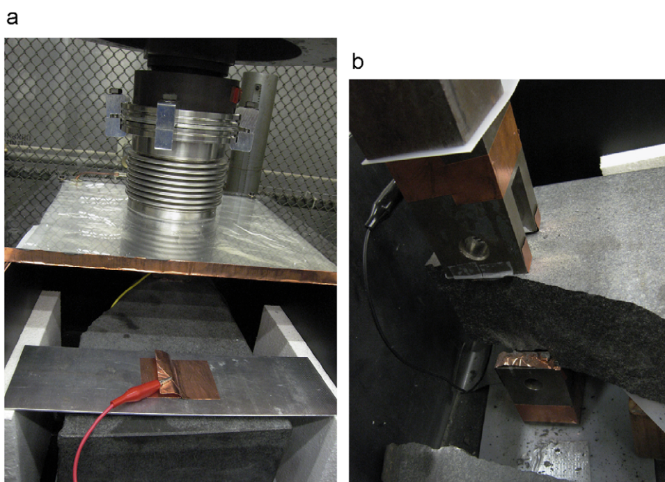
Fig. 3. (a/b): two inside views of the Faraday cage after completion of experiment #37, in which an approximately triangular portion the gabbro block split off laterally, causing the rock to only slightly tilt upon failure. (a) Position of the Al sheet used as ion collector or as capacitor place. (b) The pistons with stainless steel ball bearing stress concentrators and the polyethylene sheets.
